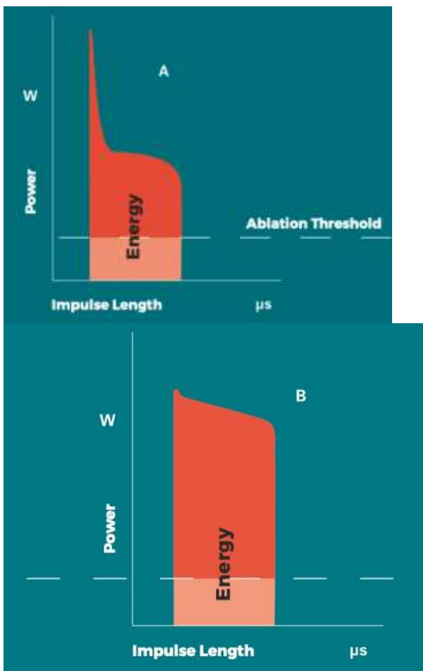
Fig. A: Single-pulse continuous-supply excited laser CO 2 (Superpulse emission). Fig. B: Single-pulse radiofrequency excited laser CO 2 (Ultrapulse emission). Radiofrequency-excited CO 2 laser sources produce greater energy above the ablation threshold (red colour) compared to continuous-supply excited CO 2 lasers, and at comparable pulse length.
